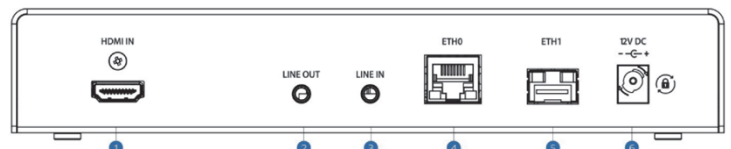
[リアパネル]
